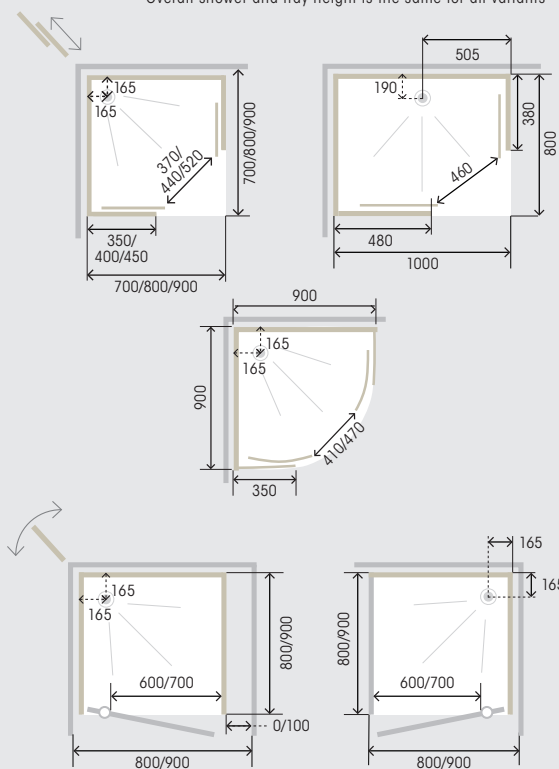
All measurements in mm
