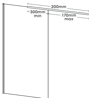
Solo 6+ Ceiling mounted mast bar, installed horizontally in a recess
