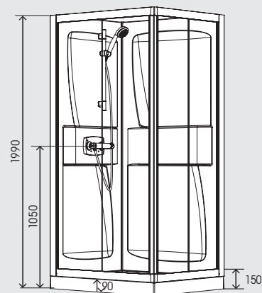
Overall shower and tray height is the same for all variants
